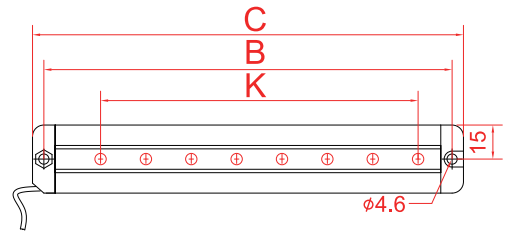
C type Dirc output ,Single screw hole fixing
