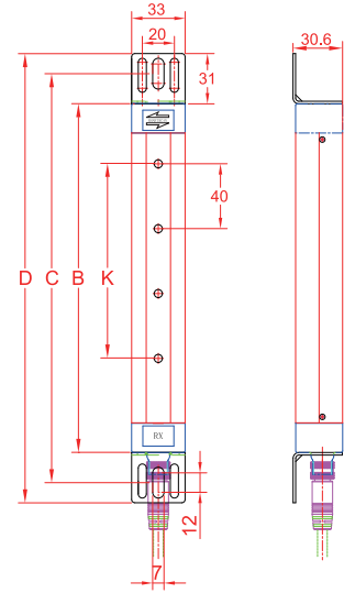
NA Dimensions
