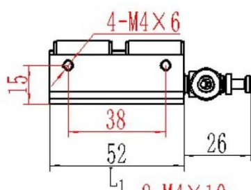
Opening and closing travel: L48mm installation dimensions
