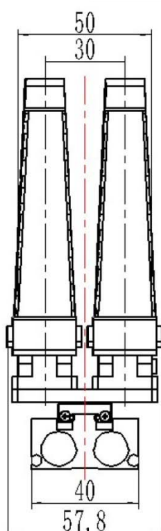
4 fingers, W30, side view
