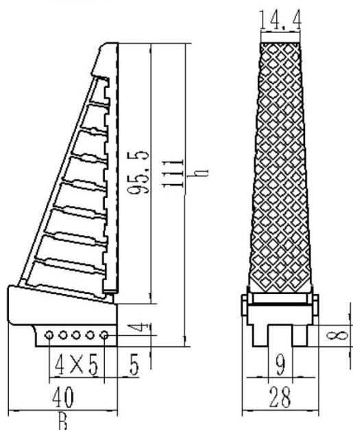
FAMR100 finger module
