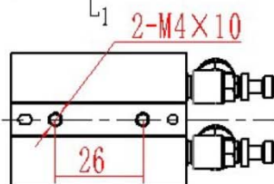
Opening and closing travel: L12mm installation dimensions
