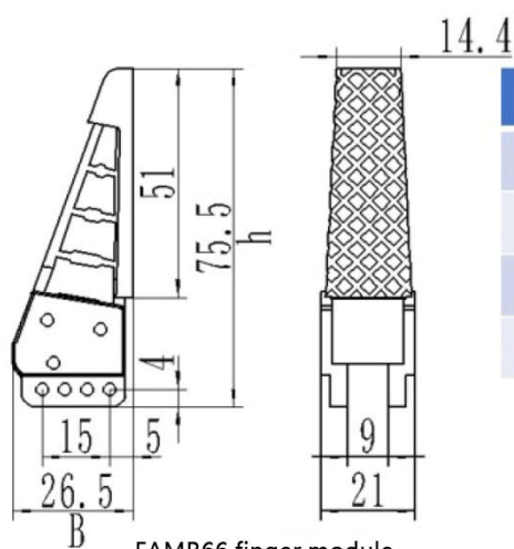
FAMR66 finger module
