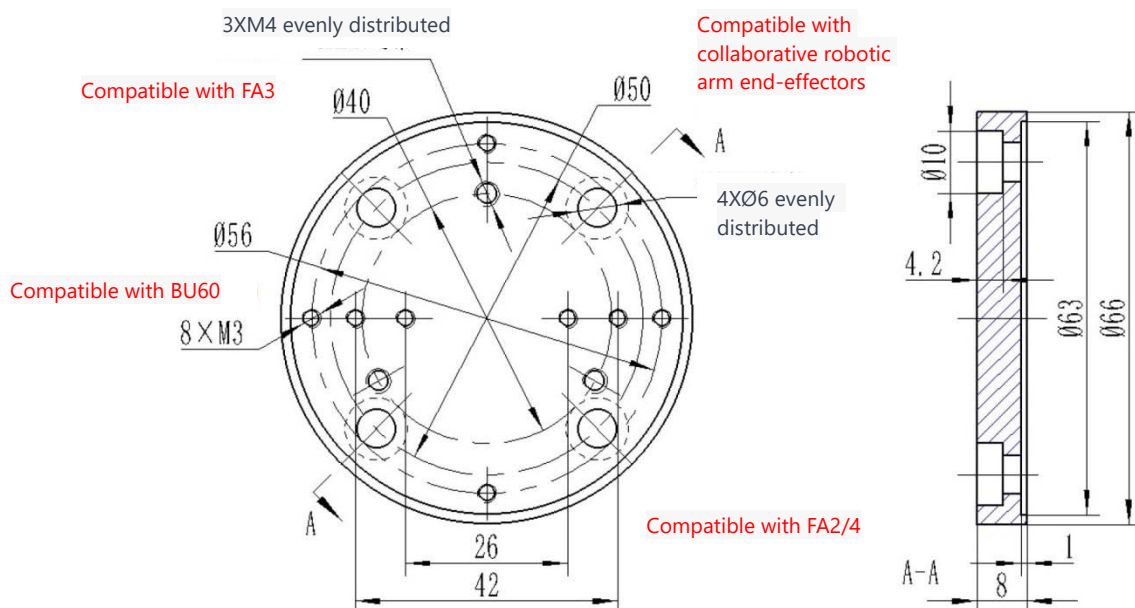
Dimensions for the FA series robotic gripper to collaborative robotic arm adapter plate
