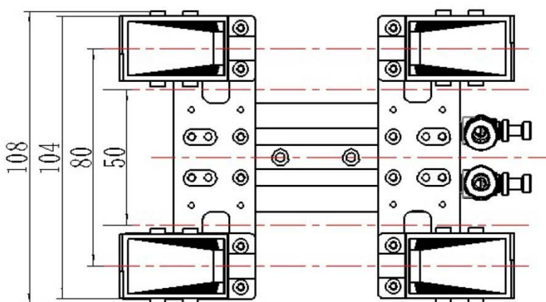
4 fingers, long board W80, top view. Finger spacing can be 80mm or 50mm, and it can also be integrated into 6 fingers or 8 fingers
