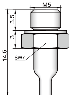
MP2-11 AN □ -A5 (M5 \times 0.8 male thread)
