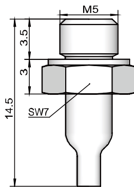
MP2-11 AN □ -A5 (M5 \times 0.8外螺紋)
