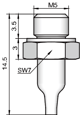
MP2-08 AN □ -A5 (M5 \times 0.8外螺紋)
